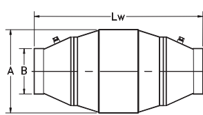
MINE-X® Welded Design (DP) DC10 to DC16
